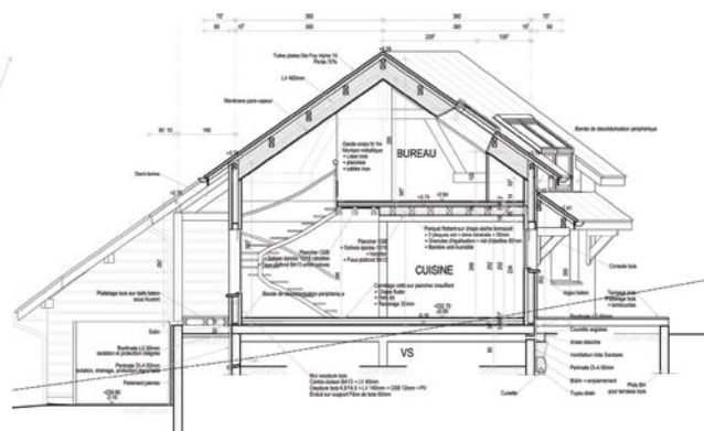
Villa ossature bois – Saint Jean Saint Nicolas (05)
