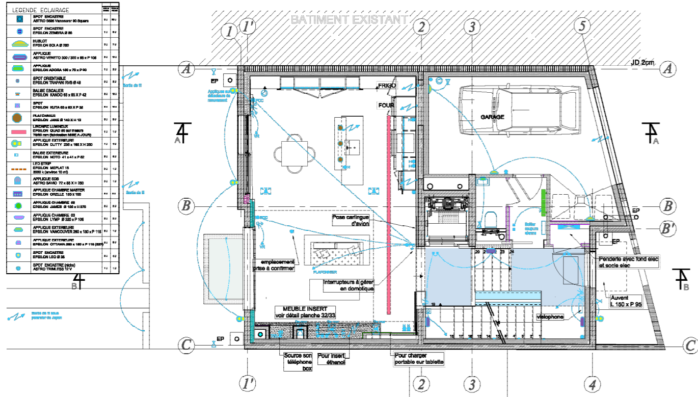
PLAN REZ DE CHUSSEE ELECTRICITE
