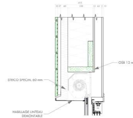
DETAIL VOLET ROULANT
