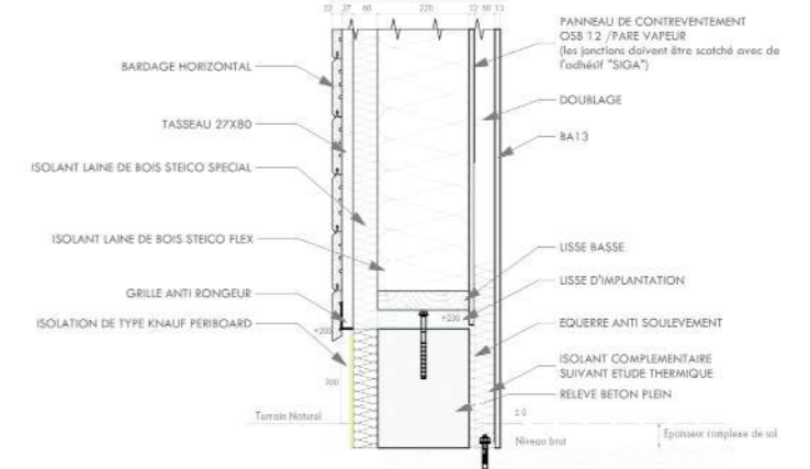
DETAIL OSSATURE BOIS
