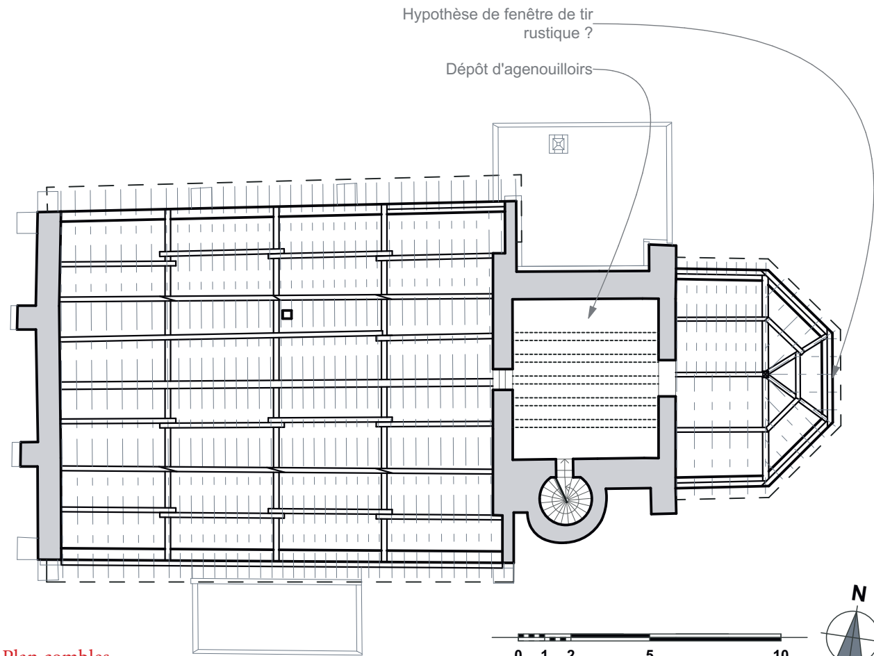
Plan comble
